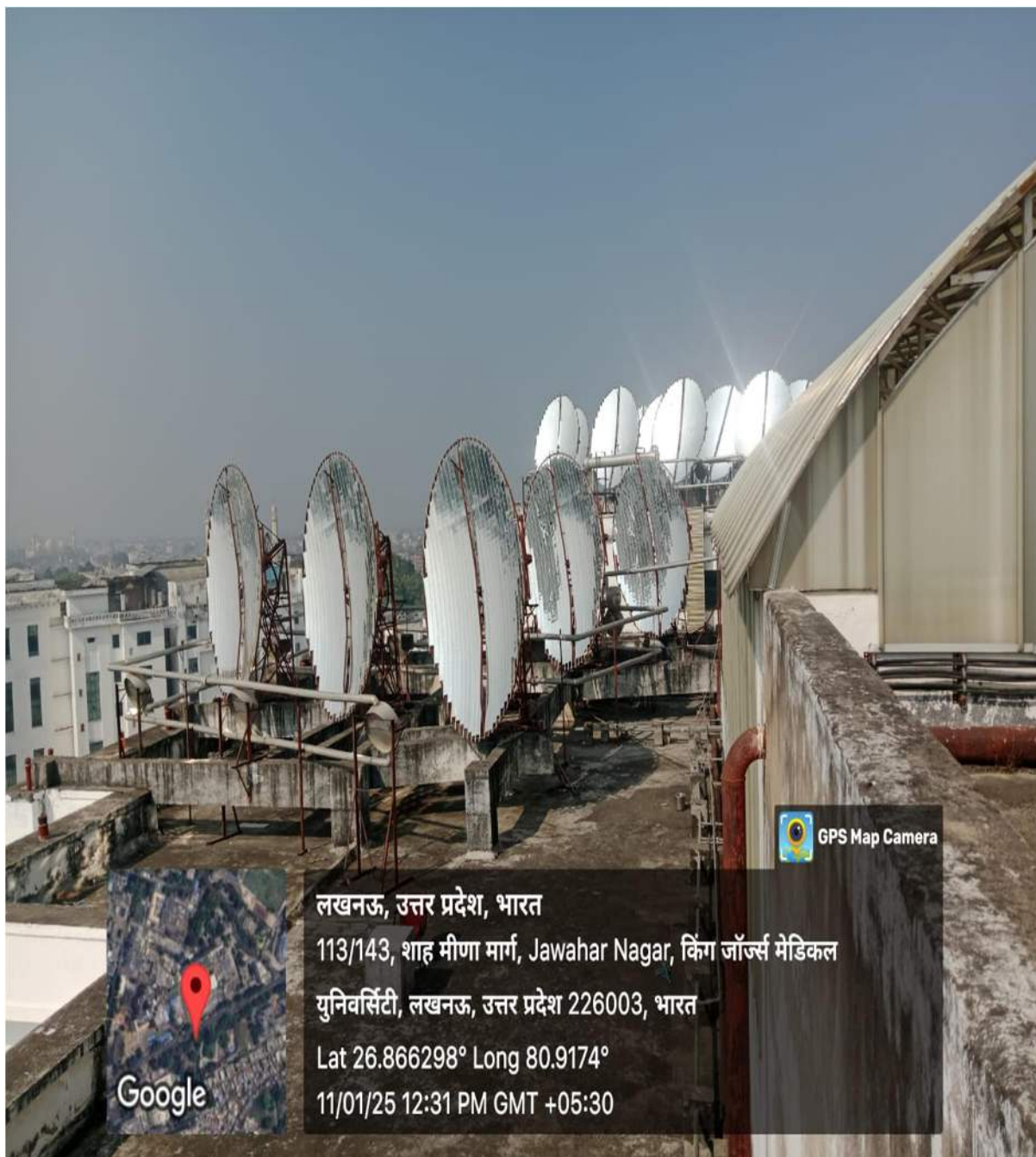
Solar paraboloids for hospital kitchen cooking by steam atop Shatabdi Hospital
