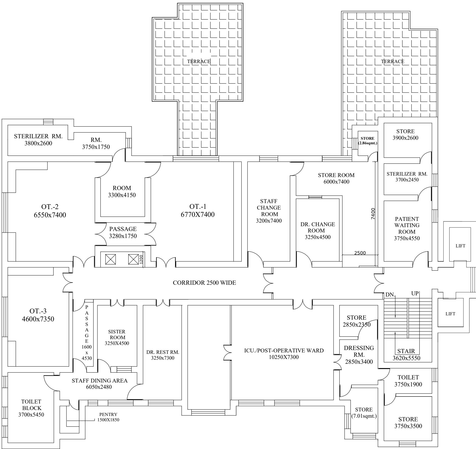
SECOND FLOOR PLAN UROLOGY DEPARTMENT KGMU. LUCKNOW
